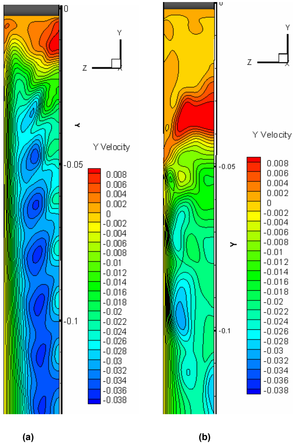
Figure 24. Instantaneous y-velocity component (a) Ri=0.0 (b) 1.05
