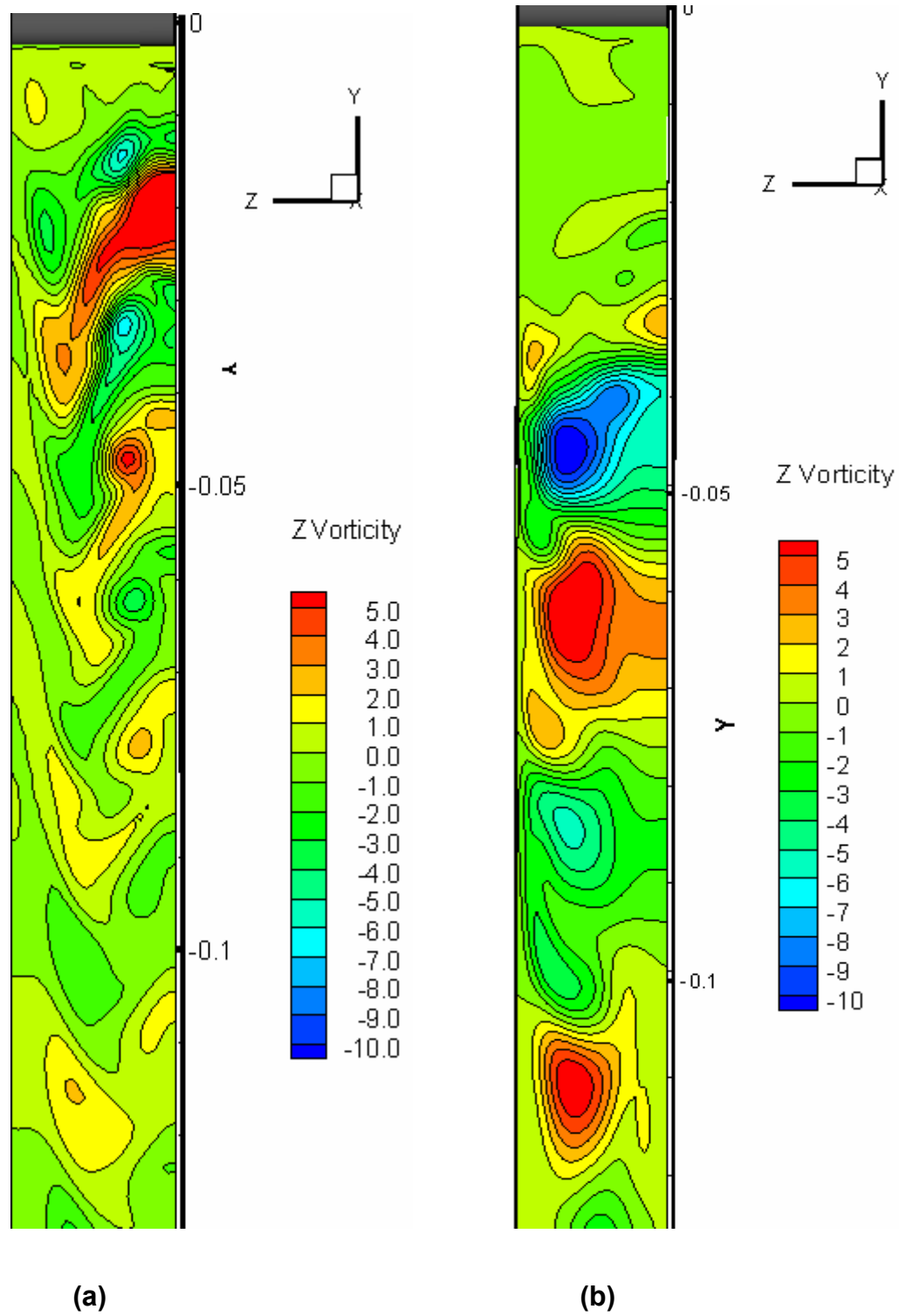
Figure 28. Instantaneous z-vorticity component (a) Ri=0.0 (b) 1.05
